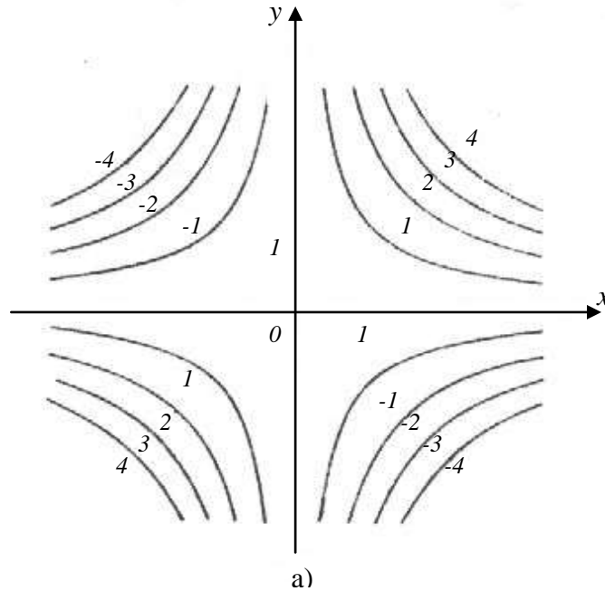
Fig. 26.1 Campo Vectorial Central
